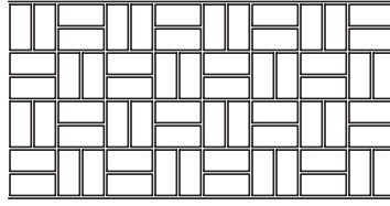
BASKET WEAVE BRICK SIZE: 3 \frac{1}{2}'' \times 7 \frac{3}{4}'' ROLL WIDTH: 33 \frac{1}{2}'' JOINT WIDTH: \frac{1}{2}''
