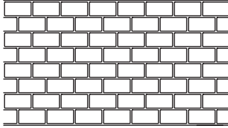
RUNNING BOND BRICK SIZE: 4'' \times 7 \frac{3}{4}'' ROLL WIDTH: 36 \frac{1}{2}'' JOINT WIDTH: \frac{1}{2}''
