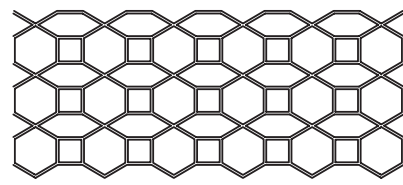
MEDITERRANEAN OCTAGON: 21" X 13 1/8" ROLL WIDTH: 32" JOINT WIDTH: 1/2"
