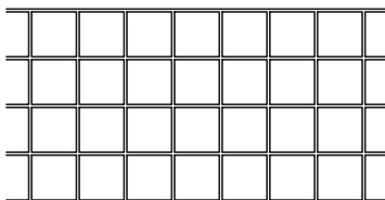
MEDIUM TILE TILE SIZE: 7 3/4" X 7 3/4" ROLL WIDTH: 33 1/2" JOINT WIDTH: 1/2"
