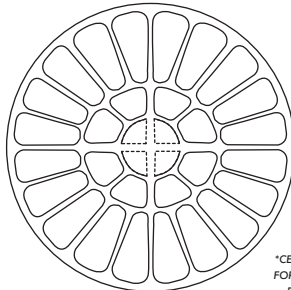
UNIVERSAL CIRCLE* DIAMETER: 2' 11 \frac{1}{2}'' JOINT WIDTH: \frac{1}{2}''
