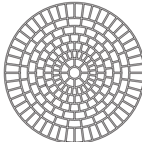
BRICK ROSETTE AVAILABLE DIAMETERS: 5' 5 \frac{1}{4}'' • 7' 2'' JOINT WIDTH: \frac{1}{2}'' • \frac{7}{8}''
