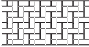
ORIGINAL HERRINGBONE BRICK SIZE: 3 \frac{1}{2}'' \times 7 \frac{3}{4}'' ROLL WIDTH: 33 \frac{1}{2}'' JOINT WIDTH: \frac{1}{2}''
