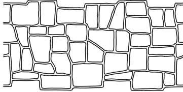
KEYSTONE LARGEST STONE SIZE: 11" X 8" ROLL WIDTH: 33" JOINT WIDTH: 1/2" - 1 1/4"
