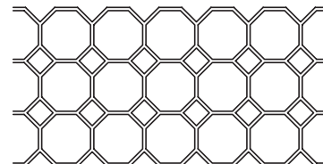
10" OCTAGON TILE OCTAGON DIAMETER: 10 1/4" ROLL WIDTH: 33 1/2" JOINT WIDTH: 11/16"
