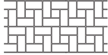
FLANDERS WEAVE FULL BRICK SIZE: 4 \frac{7}{8}'' \times 10 \frac{1}{2}'' ROLL WIDTH: 33'' JOINT WIDTH: \frac{1}{2}''
