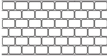
COBBLESTONE BRICK SIZE: 4 15/16" X 7 7/8" ROLL WIDTH: 33" JOINT WIDTH: 1/2"
