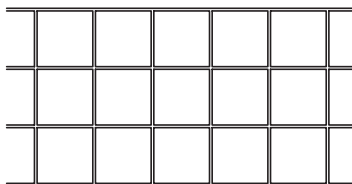
LARGE TILE TILE SIZE: 10 1/2" X 10 1/2" ROLL WIDTH: 33 1/2" JOINT WIDTH: 1/2"
